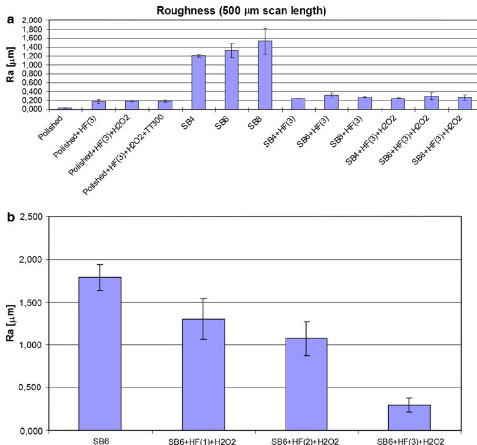
Fig. 3 Surface roughness of samples with different surface treatments
