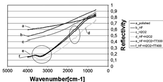
Fig. 6 FTIR spectra of samples with different surface treatments
