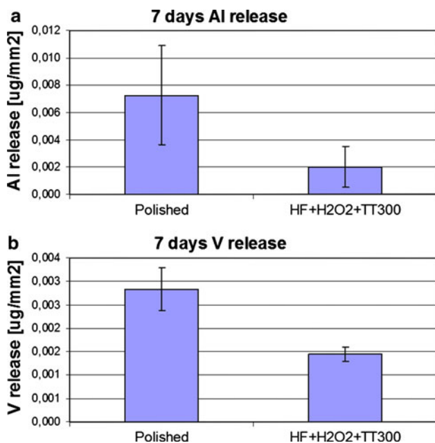
Fig. 11 Ion release after 1 week in SBF from Ti6Al4V samples before and after HF + H 2 O 2 + TT300 treatment. a Al, b V
