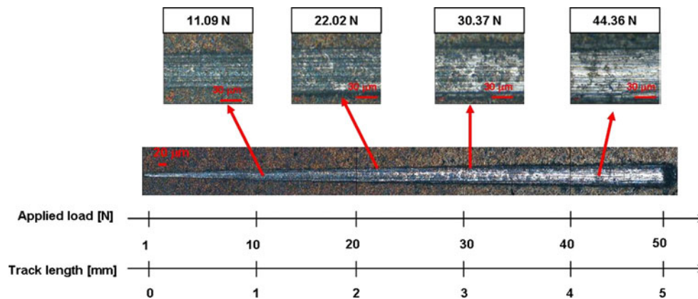
Fig. 9 Scratch track and magnification of critical loads point for Ti6Al4V + HF + H 2 O 2 + TT300 sample
