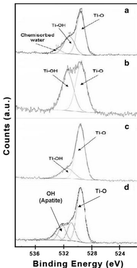
Fig. 7 XPS spectra of a polished, b polished + HF + H 2 O 2 sample; c polished + HF + H 2 O 2 + TT300 sample and d polished + HF + H 2 O 2 + TT400 sample after 15 days in SBF
